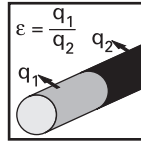
Emissionsgrad \epsilon [-]
